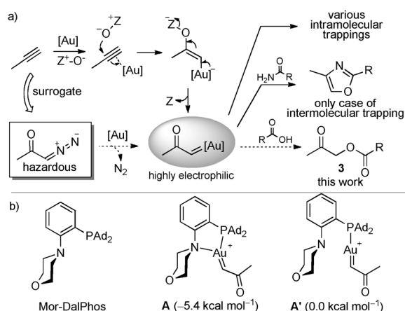
Scheme 1. a) Trapping \alpha -oxo gold carbenes generated by intermolecular alkyne oxidation using internal and external nucleophiles. b) Mor-DalPhos and the previously calculated relative energies ( \text{kcal mol}^{-1} ) of the corresponding gold carbene species. The PBE1PBE/6-311 + G** level of theory was used. [6]
